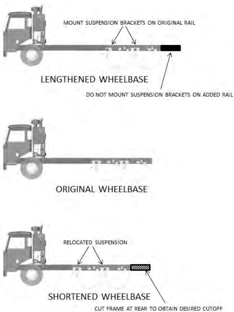
FIGURE 5-1. Wheelbase Customization
