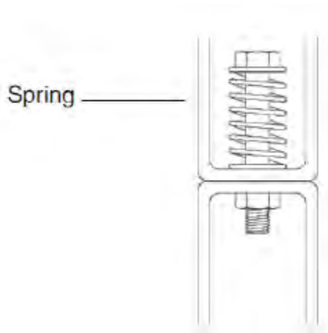
FIGURE 4-4. Mounting Brackets
