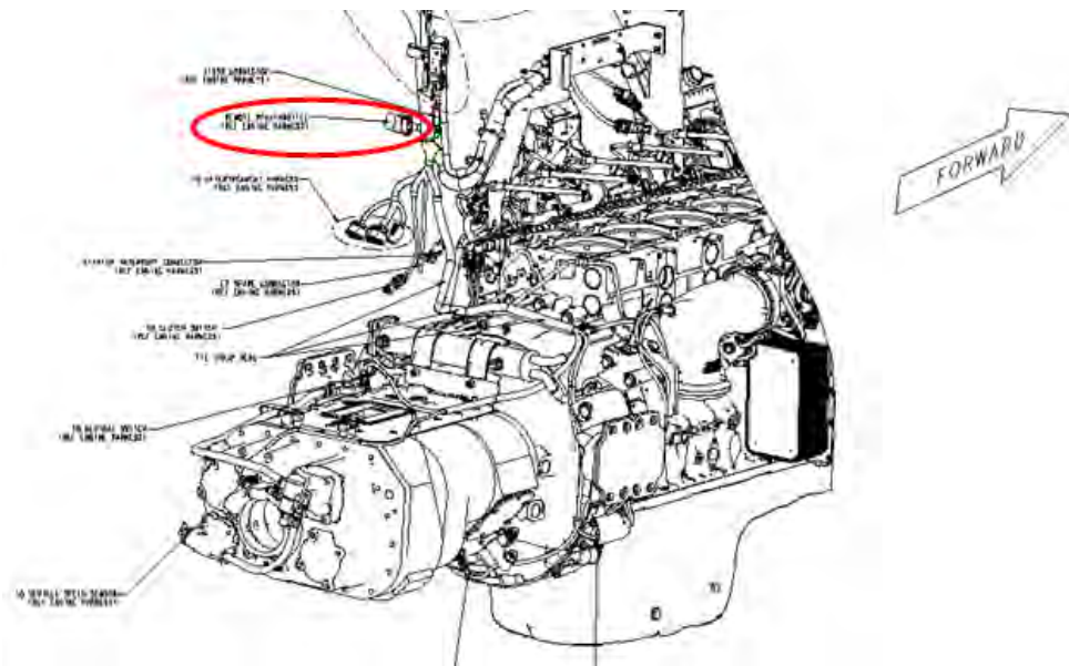
FIGURE 7-9. Connector Location
