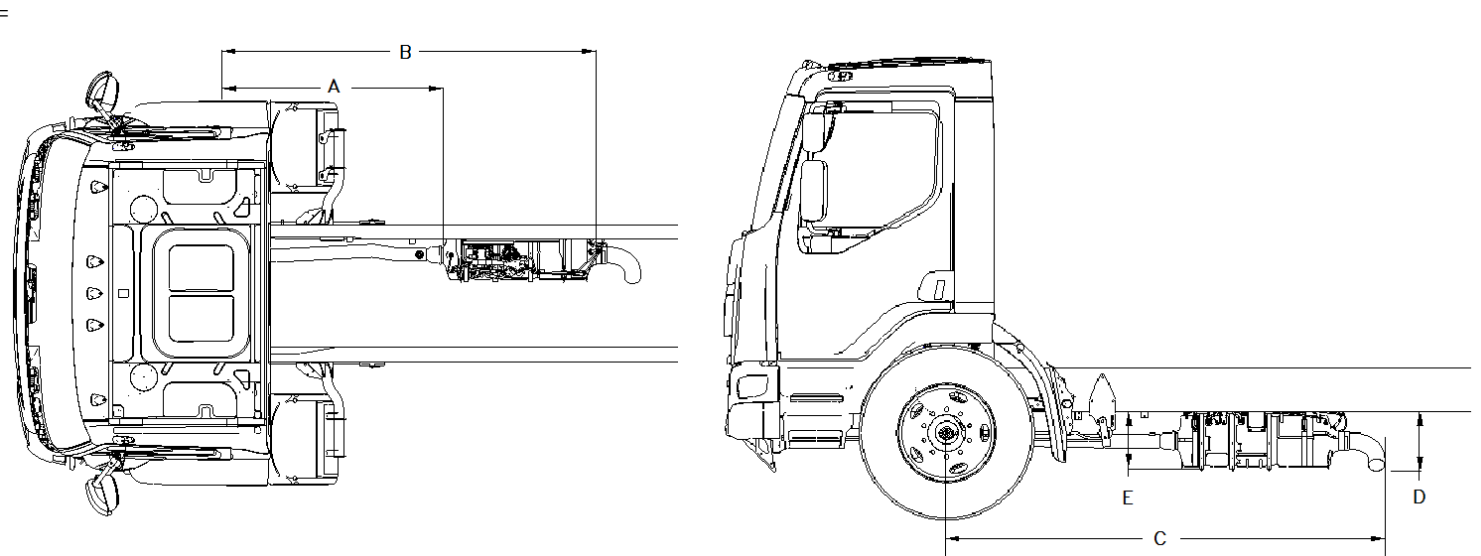
Figure 3-9.1 Model 220 Exhaust Measurements
