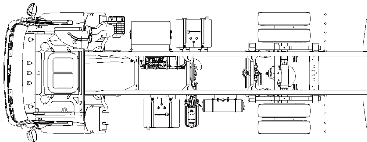
Figure 3-6.1 Model 220 Crossmember Locations
