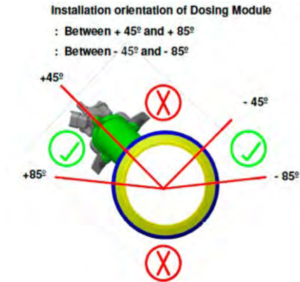
Figure 4-4 Orientation of Dosing Module
